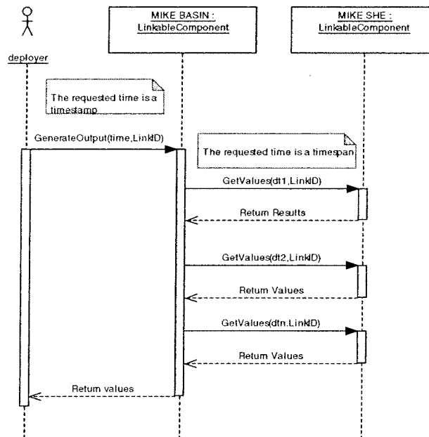
Figure 3. Simulation process for the uni-linked models.
