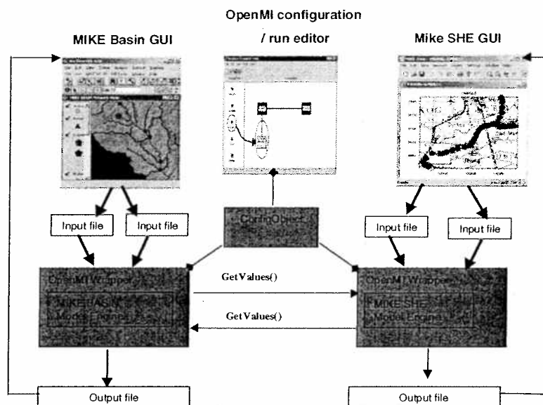
Figure 1. MIKE BASIN and MIKE SHE linked through the OpenMI system.
