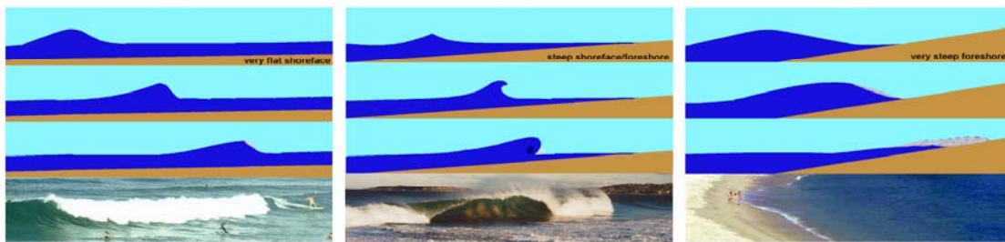
Figure 4. Wave breaking on the shoreface: spilling, plunging and surging. (From Mangor 2004).
