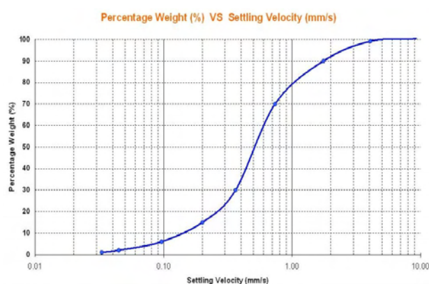
Figure 7. Example sediment fall velocity distribution from Owen Tube test of fine material content of reclamation fill
