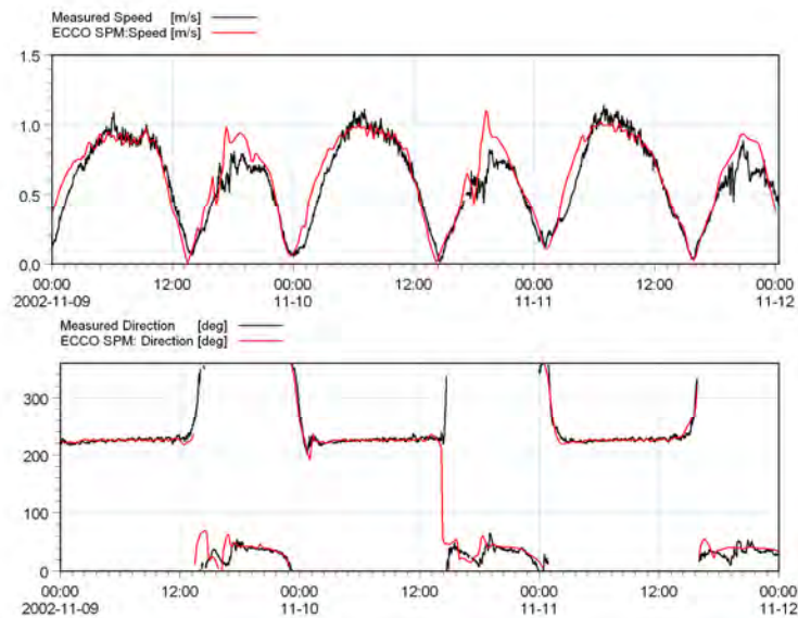
Figure 4. Example performance of DHI's Singapore Straits current forecast model. RMS error on current speed at presented validation point = 0.09m/s
