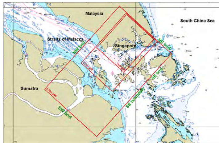
Figure 3. DHI's Singapore Straits regional 675m grid model with nested intermediate 225m grid and local 75m grid sub-domain models
